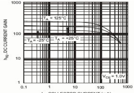
Fig. 2 Typical DC Current Gain vs Collector Current
