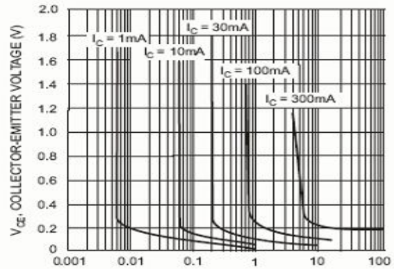
Fig. 4 Typical Collector Saturation Region
