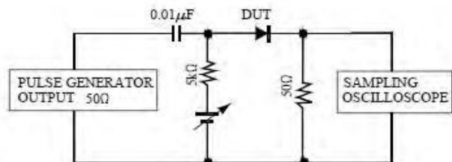
Reverse Recovery Time Measurement Circuit
